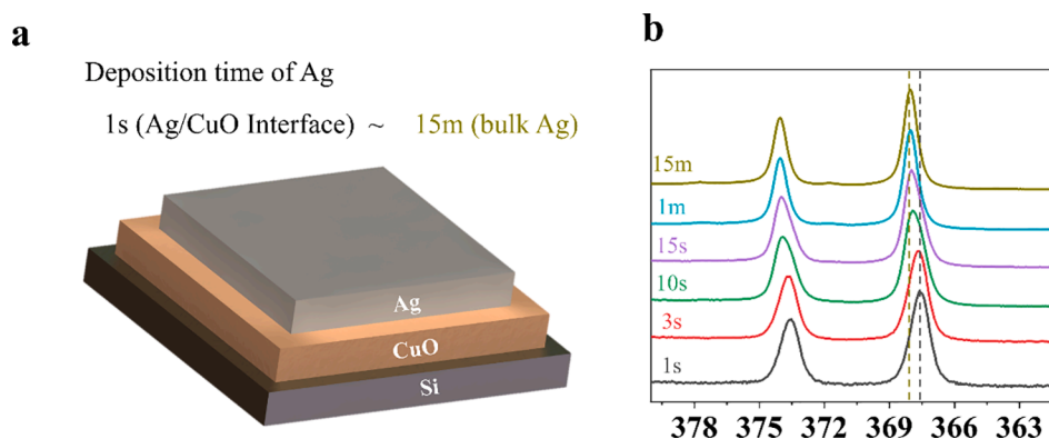
Fig. 7. (a) Scheme of Ag/CuO film on Si wafer (b) XPS Ag 3d peaks of Ag/CuO on Si wafer at different Ag deposition times.
