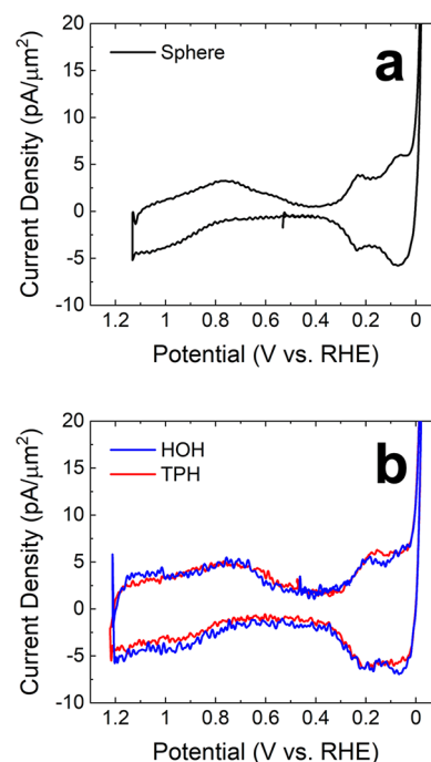
Figure 6. (a) An H CV for spherical single Pt NP. (b) H CVs for TPH and HOH single Pt NPs. The CVs were obtained in 0.5 M \text{H}_2\text{SO}_4 . The scan rate was 0.40 V/s, and the data were smoothed using the (a) 45-point and (b) 25-point FFT filters in OriginLab. The unsmoothed data are provided in Figures S7b and S7c in the SI.
