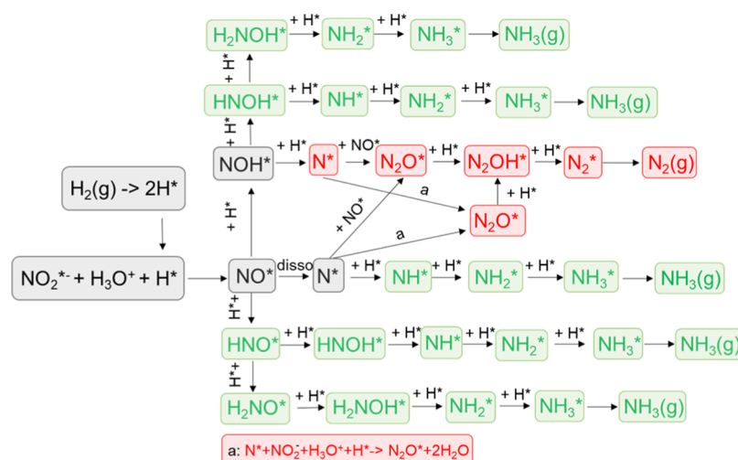
Figure 1. Catalytic reaction pathways for nitrite reduction with hydrogen gas as the reducing agent. The formation of water in the reactions is not shown.
