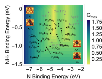
Figure 4. Volcano activity plot for nitrite reduction through the \text{NH}_3 formation pathways, with triatomic ensembles ( \text{Y}_3 , \text{X}_1\text{Y}_2 , \text{X}_2\text{Y}_1 , and \text{X}_3 , \text{X} = \text{Ir} and \text{Pt} and \text{Y} = \text{Cu} , \text{Au} , and \text{Ag} ) of the surface alloys on \text{Y} (111). The \text{X}_1\text{Y}_2 , \text{X}_2\text{Y}_1 , and \text{X}_3 triatomic ensembles were modeled as an \text{X} (111) surface, respectively, replaced by 1, 2 (twofold), and 3 (threefold) \text{X} atoms. Insets show the surface alloy models considered for the calculations: yellow and black spheres represent the \text{Y} and \text{X} atoms, respectively. The red triangles represent the triatomic ensembles as the binding sites.
